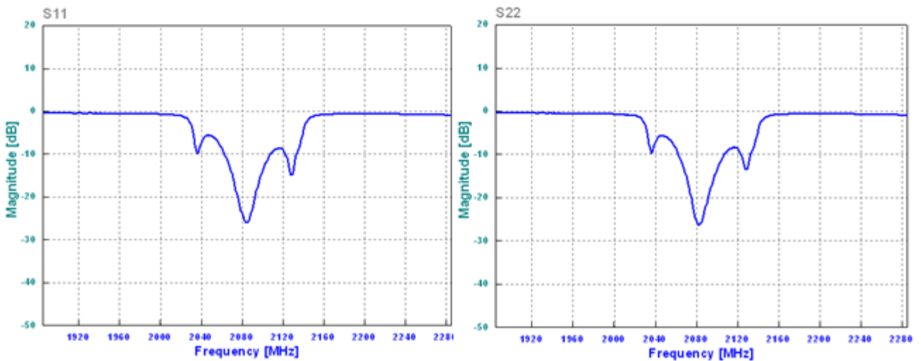
Return Loss
