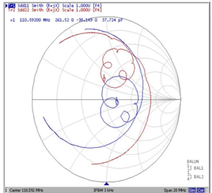
Smith Chart
