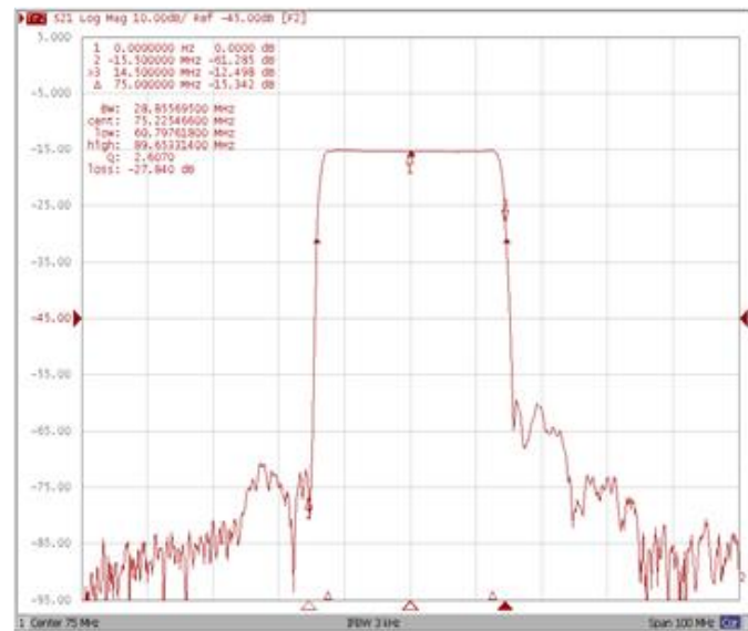
Relative Attenuation
