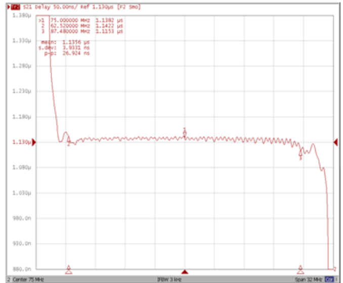
Group Delay Variation Fo±12.48MHz
