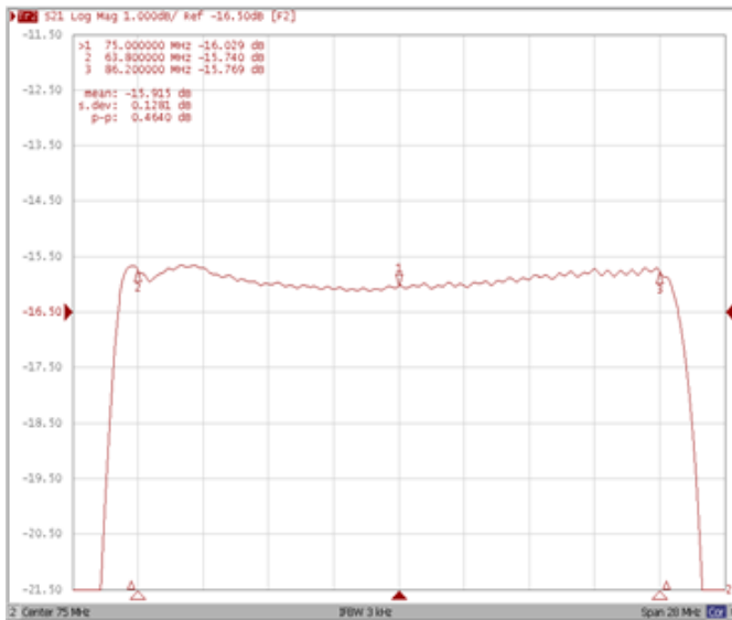
Ripple Variation Fo±11.2MHz
