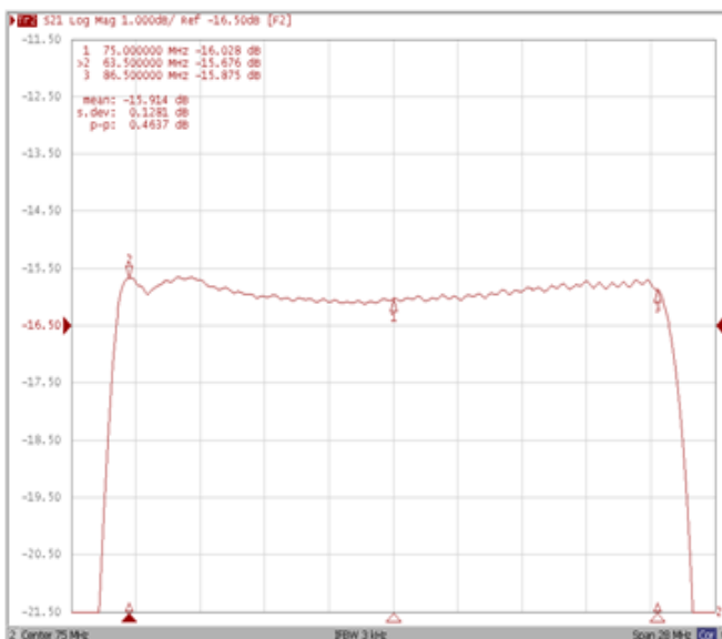
Ripple Variation Fo±11.5MHz
