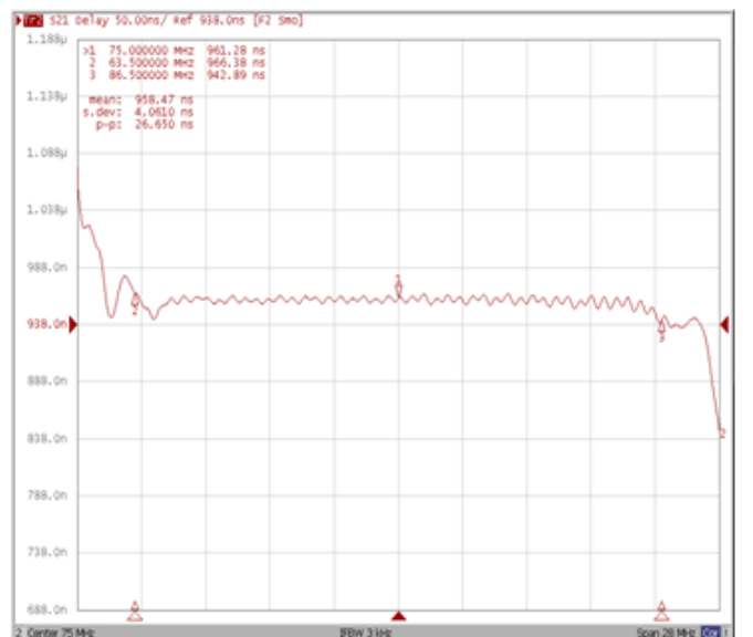
Group Delay Variation Fo±11.5MHz
