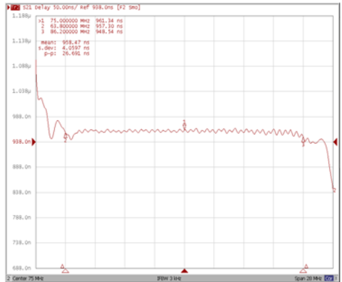
Group Delay Variation Fo±11.2MHz
