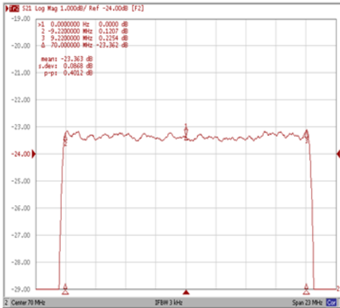
Ripple Variation Fo±9.22 MHz
