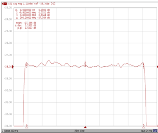
Ripple Variation Fo±9.80MHz
