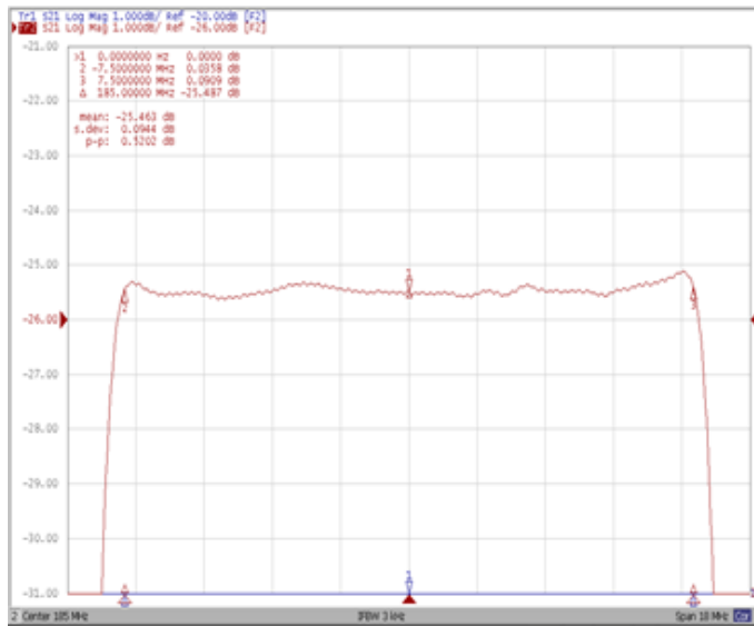
Ripple Variation Fo±7.5MHz
