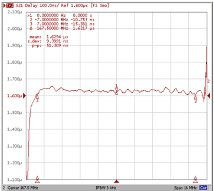
Group Delay Variation Fo±7.00MHz
