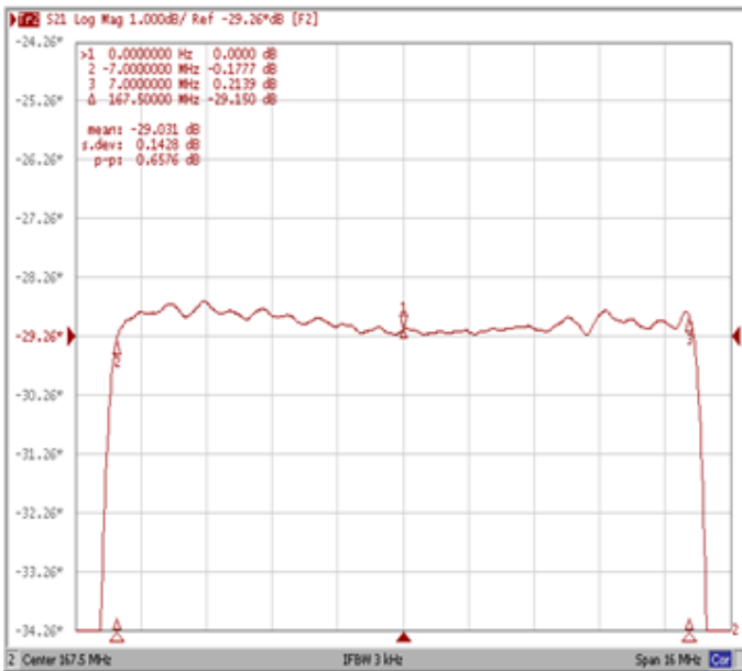
Ripple Variation Fo±7.00MHz
