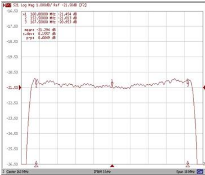
Ripple Variation F_o \pm 7.5 MHz
