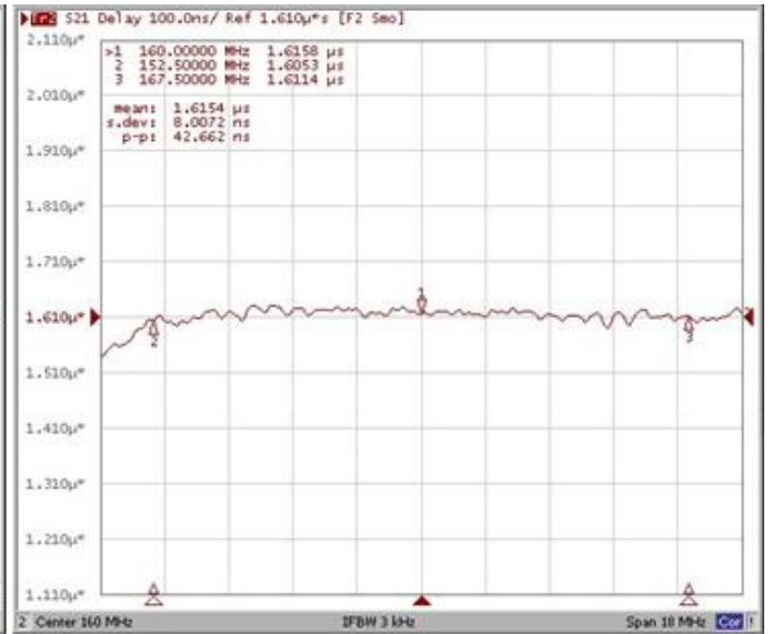
Group Delay Variation F_o \pm 7.5 MHz
