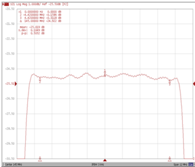
Ripple Variation Fo±4.42MHz
