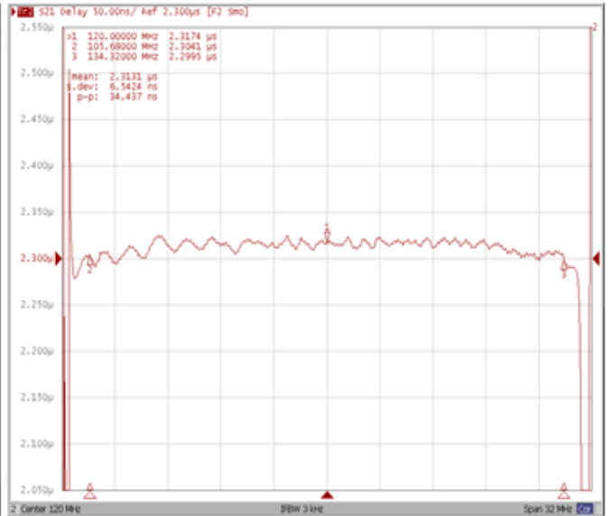
Group Delay Variation Fo±14.32 MHz
