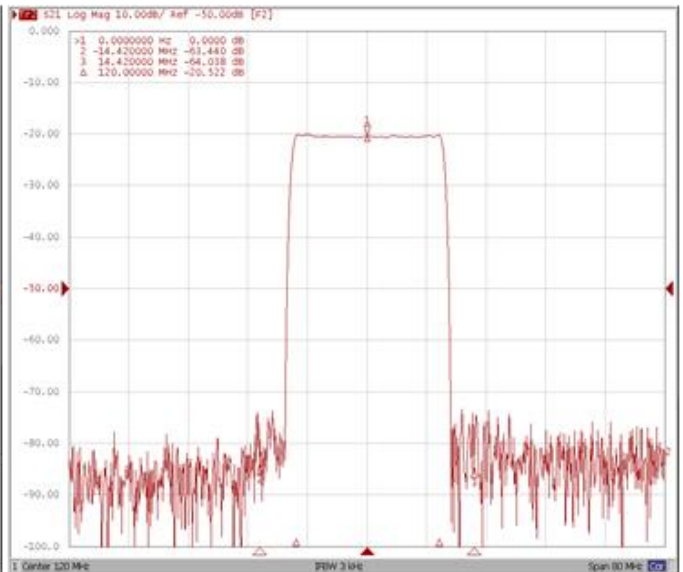
Attenuation Fo±14.42MHz
