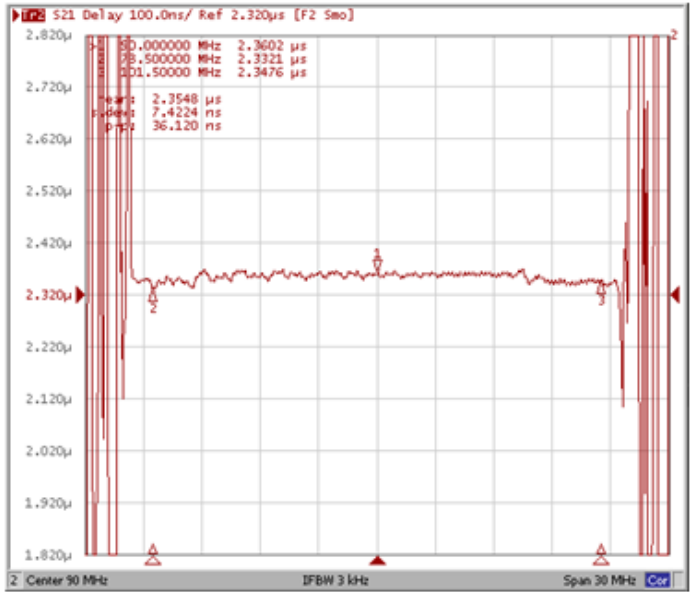
Group Delay Variation Fo±11.50MHz
