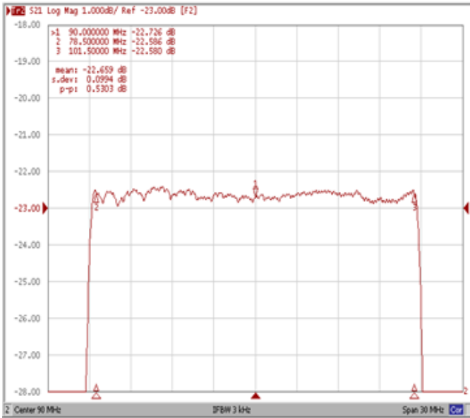
Ripple Variation Fo±11.50MHz
